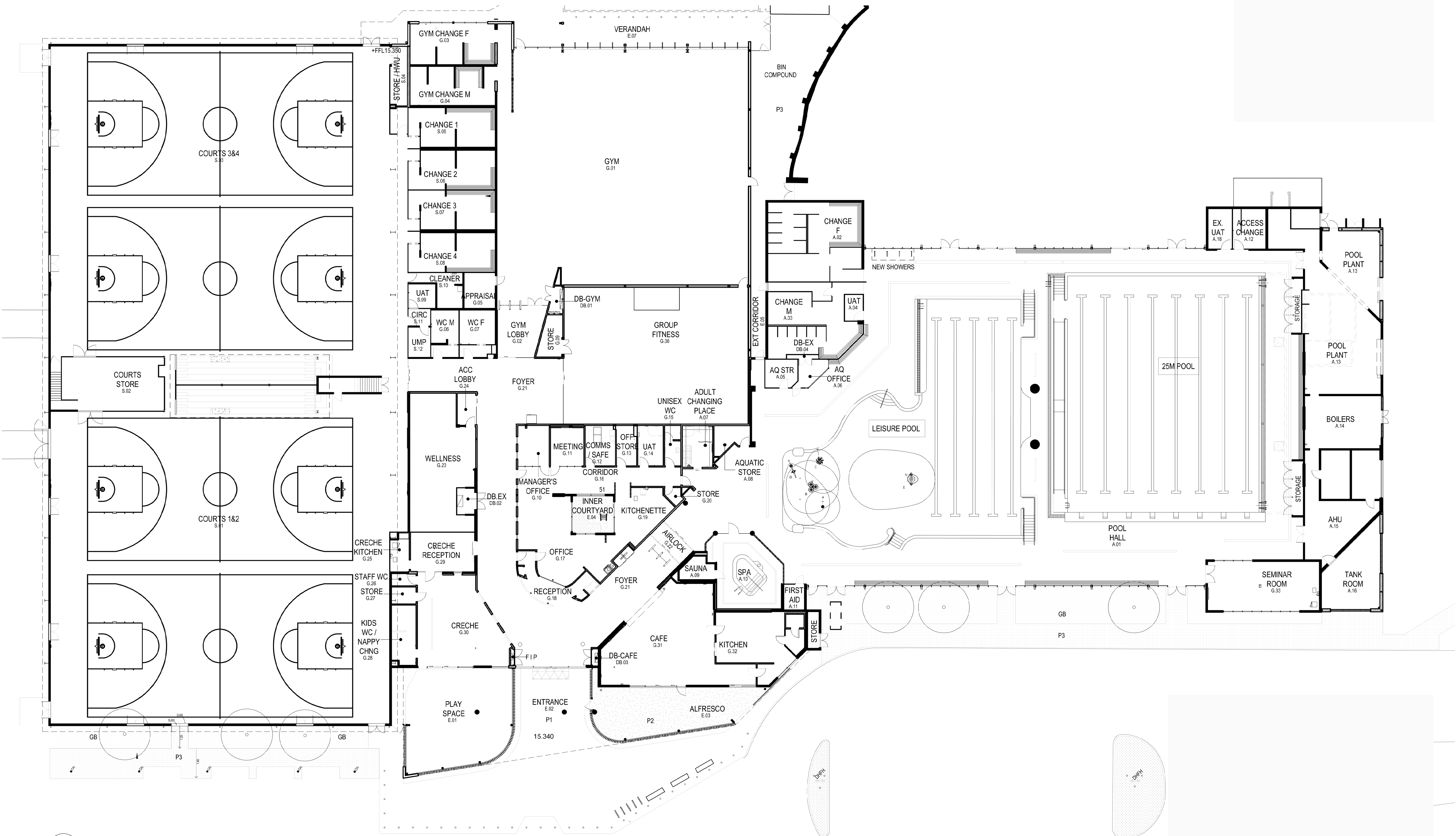
1 CLEAN OPERATIONS 1:200
